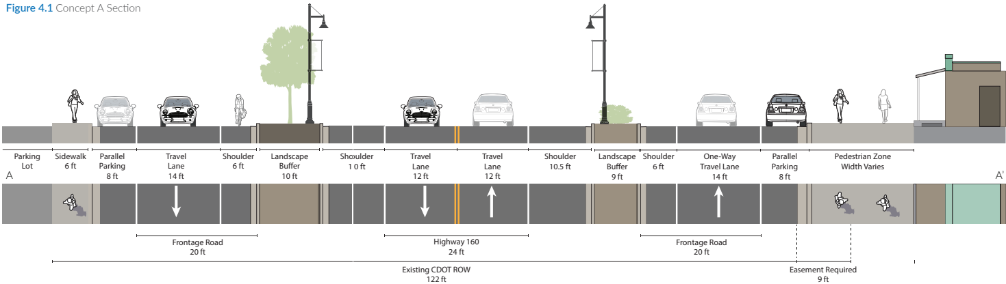
Figure 4.1 Concept A Section
