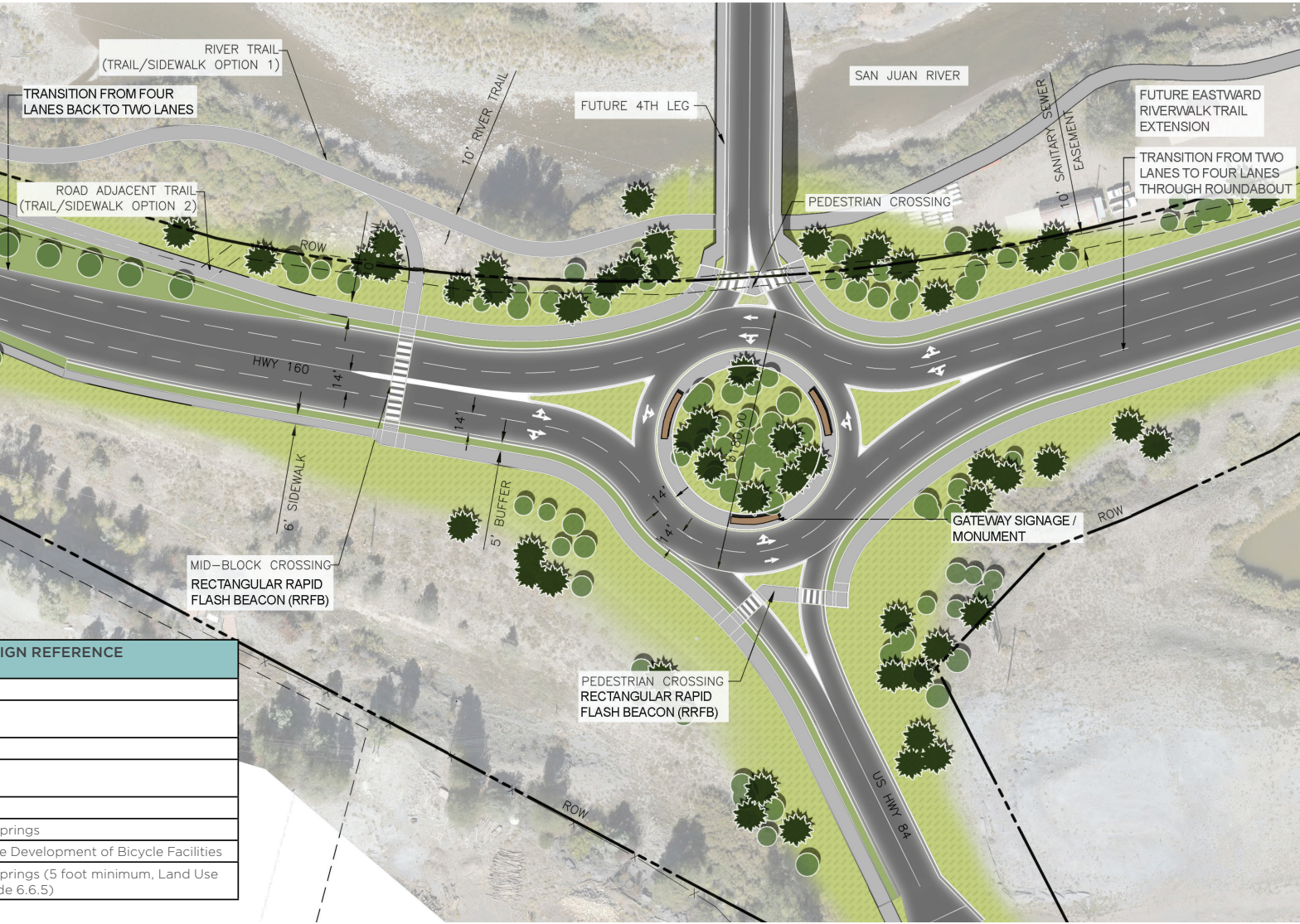
Figure 4.3 Highway 160/84 Proposed Roundabout
