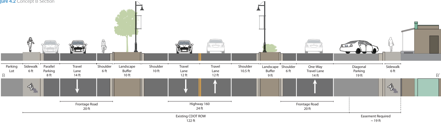
Figure 4.2 Concept B Section
